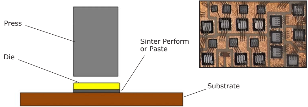
Multi-stem pressing system, able to reach every single component on the substrate.
